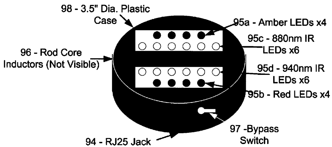
Spot Treatment Multiple Energy Assembly
