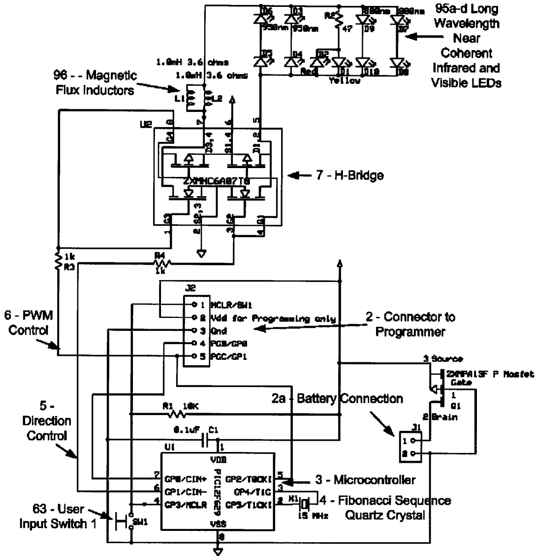
Integrated EnergyWave Therapy Device - Alternative Embodiment
