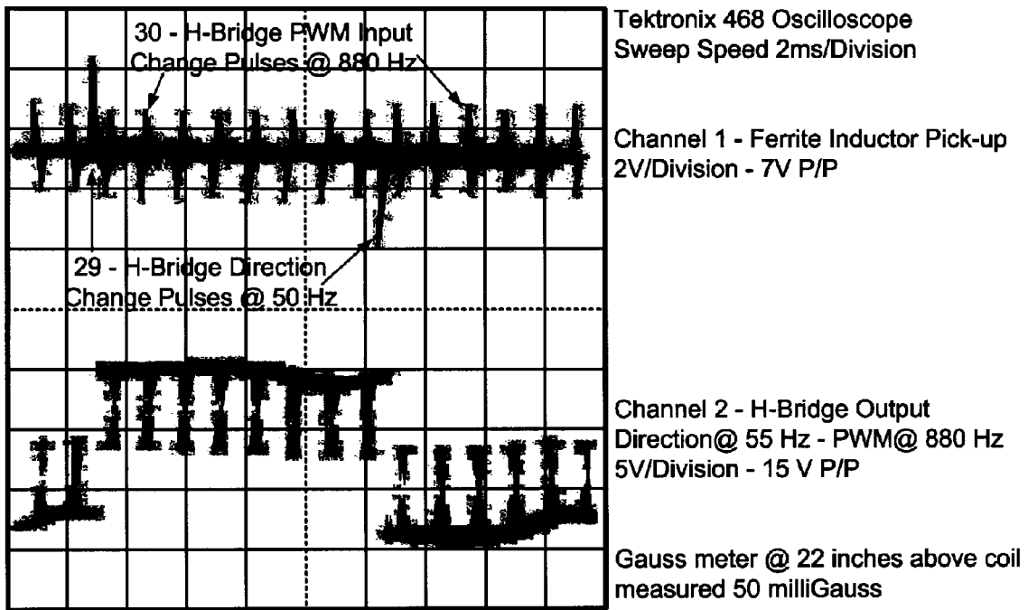
Demonstration of Multiple Simultaneous Extremely Low Frequency Waveforms Capability Using an H-Bridge with PWM and Direction Inputs
