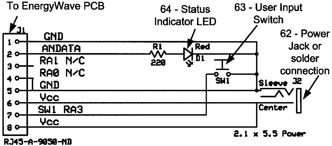
Single LED User Interface Schematic
