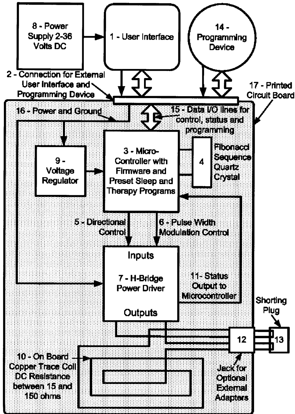
Block Diagram of EnergyWave Therapy Device
