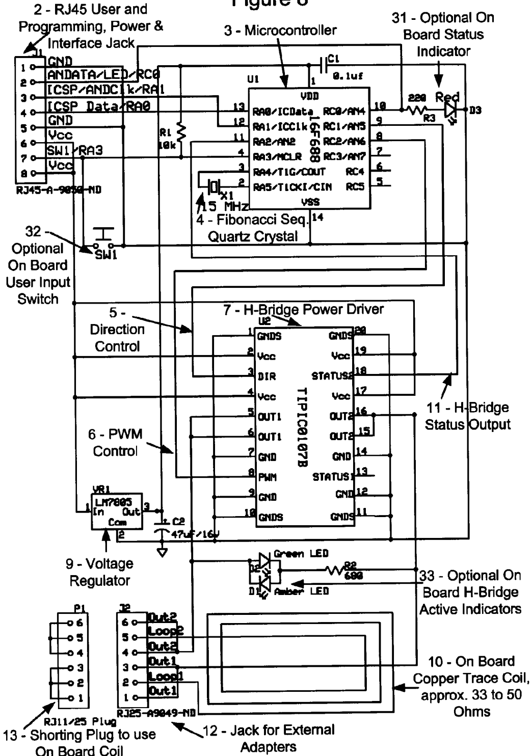
Schematic of EnergyWave Therapy Device, Preferred Embodiment
