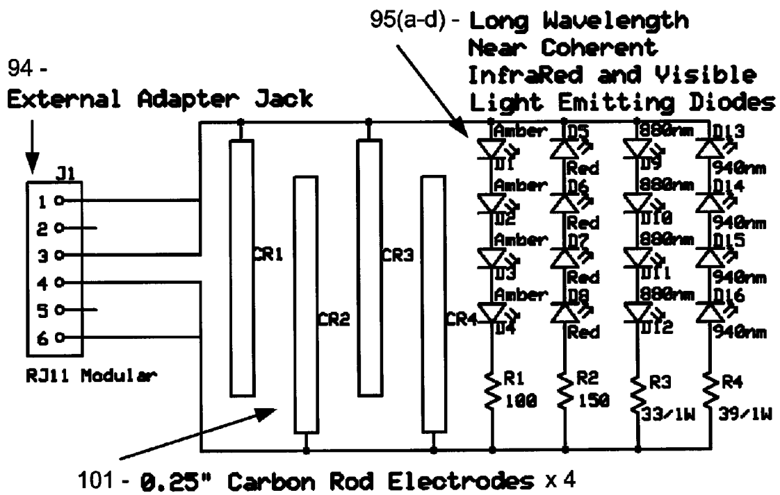
Water Foot-bath Multiple Energy Attachment
