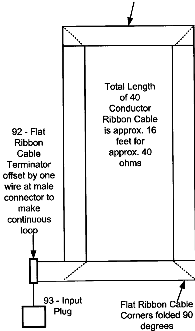
Sleep Mat Flat Coil
