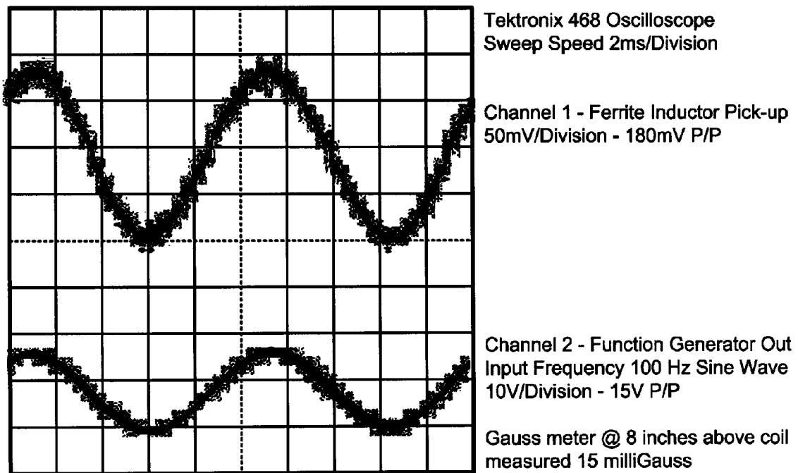
Capture of Resultant Inductance and Magnetic Flux with Sinusoidal Wave Driven Coil
